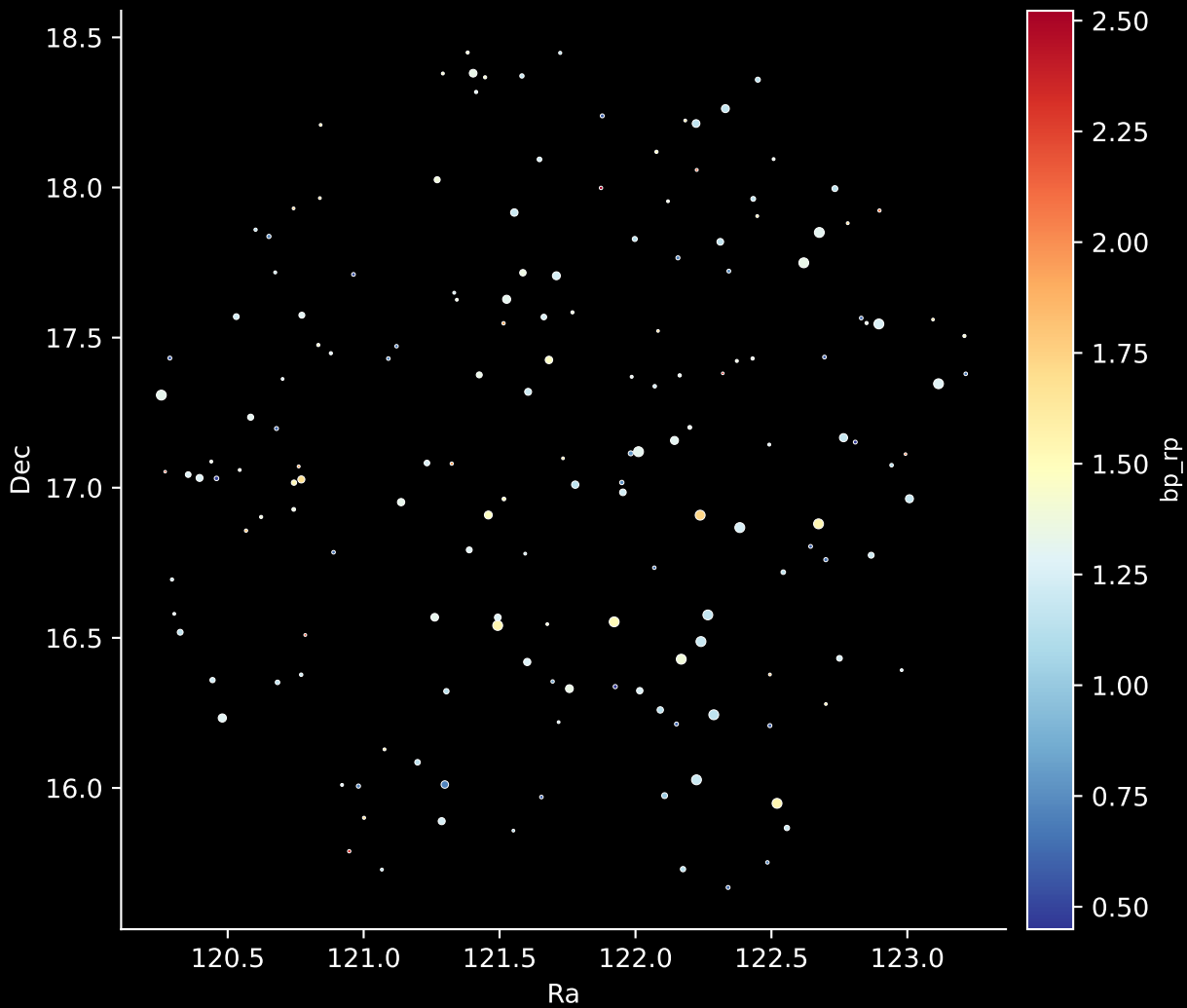
APOGEE DR17 Field: [135-45] Stars: 166
