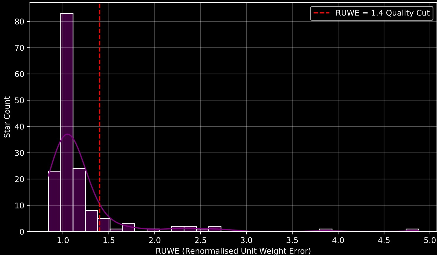
GAPOGEE DR17 Field [135-45] RUWE Distribution (n= 157)
