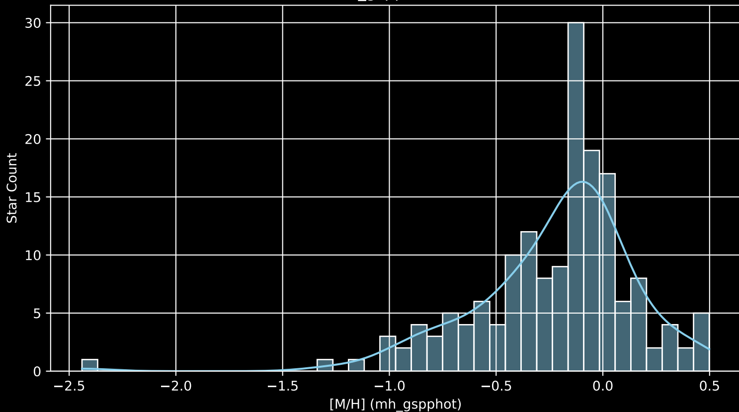
APOGEE DR17 Field: [135-45 [M/H] (mh_gspphot) (n= 166)
