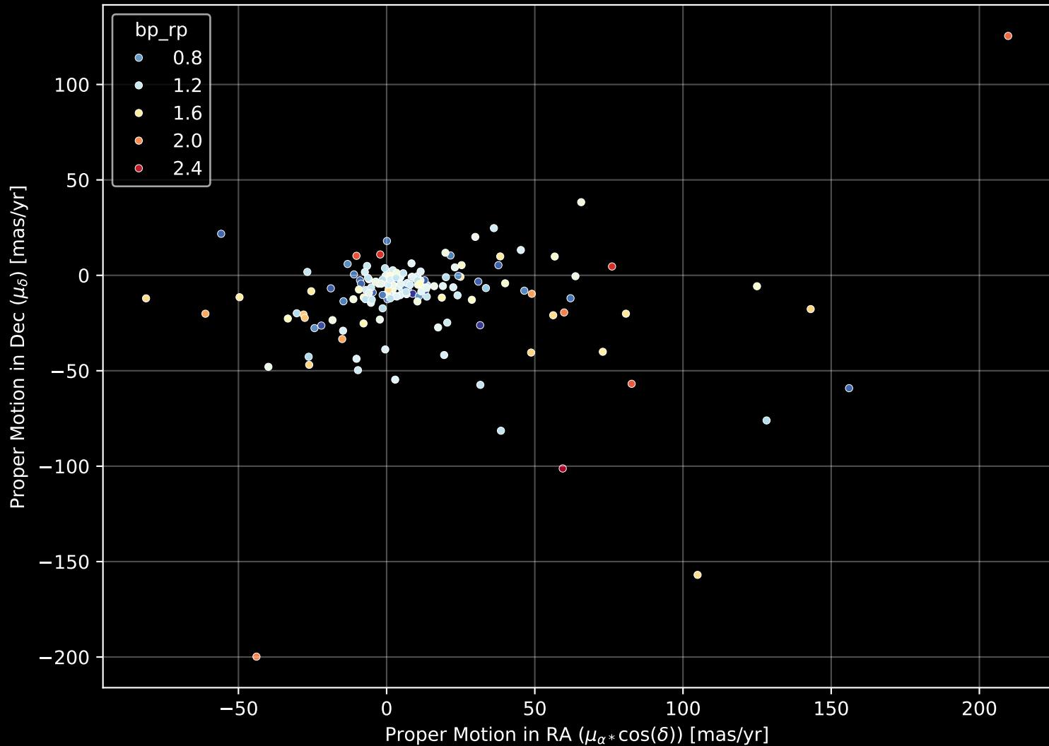
APOGEE DR17 Field: [135-45] Proper Motion Diagram (n= 166)
