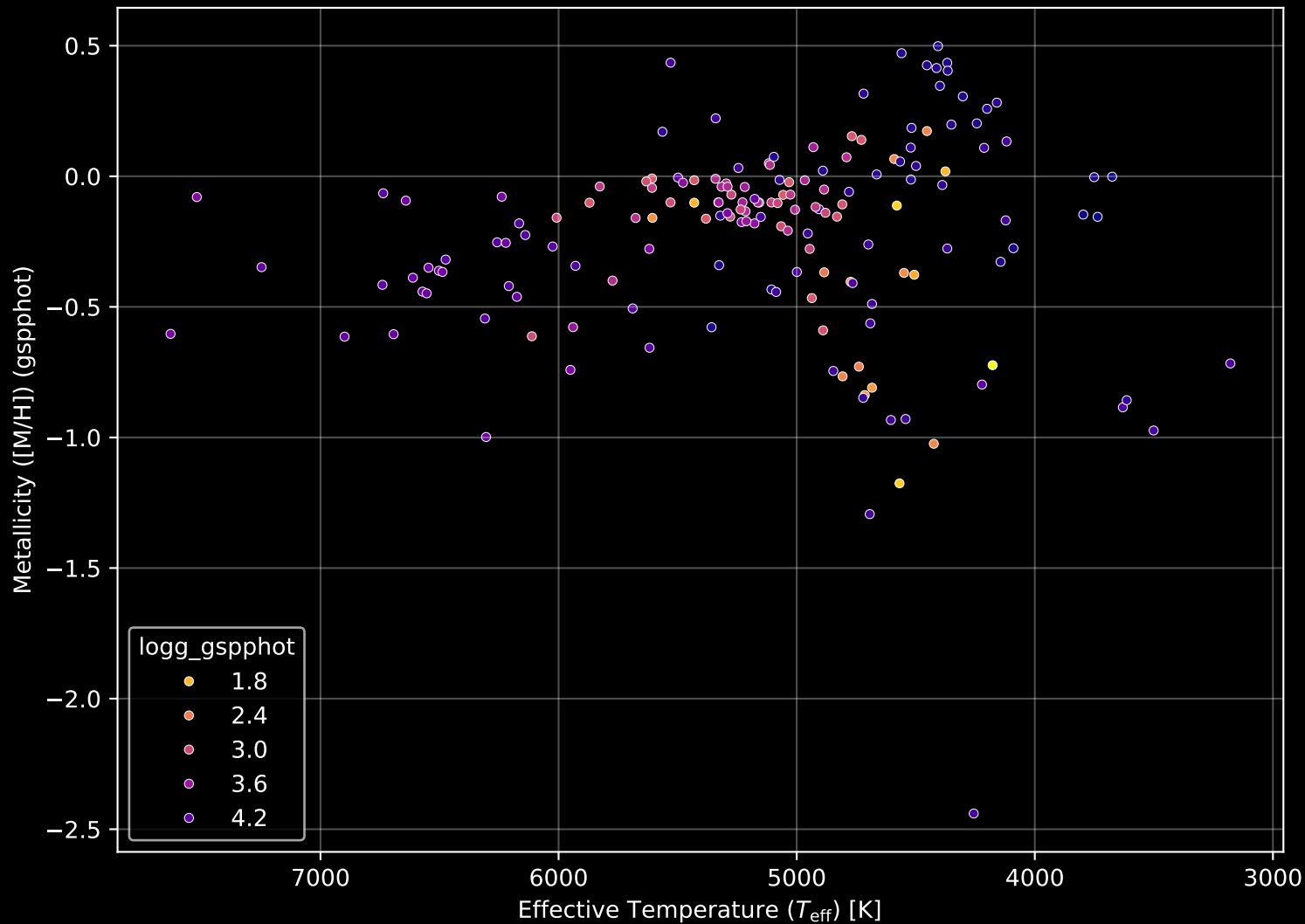
APOGEE DR17 Field: [135-45] Stellar Population Parameters (n= 166)
