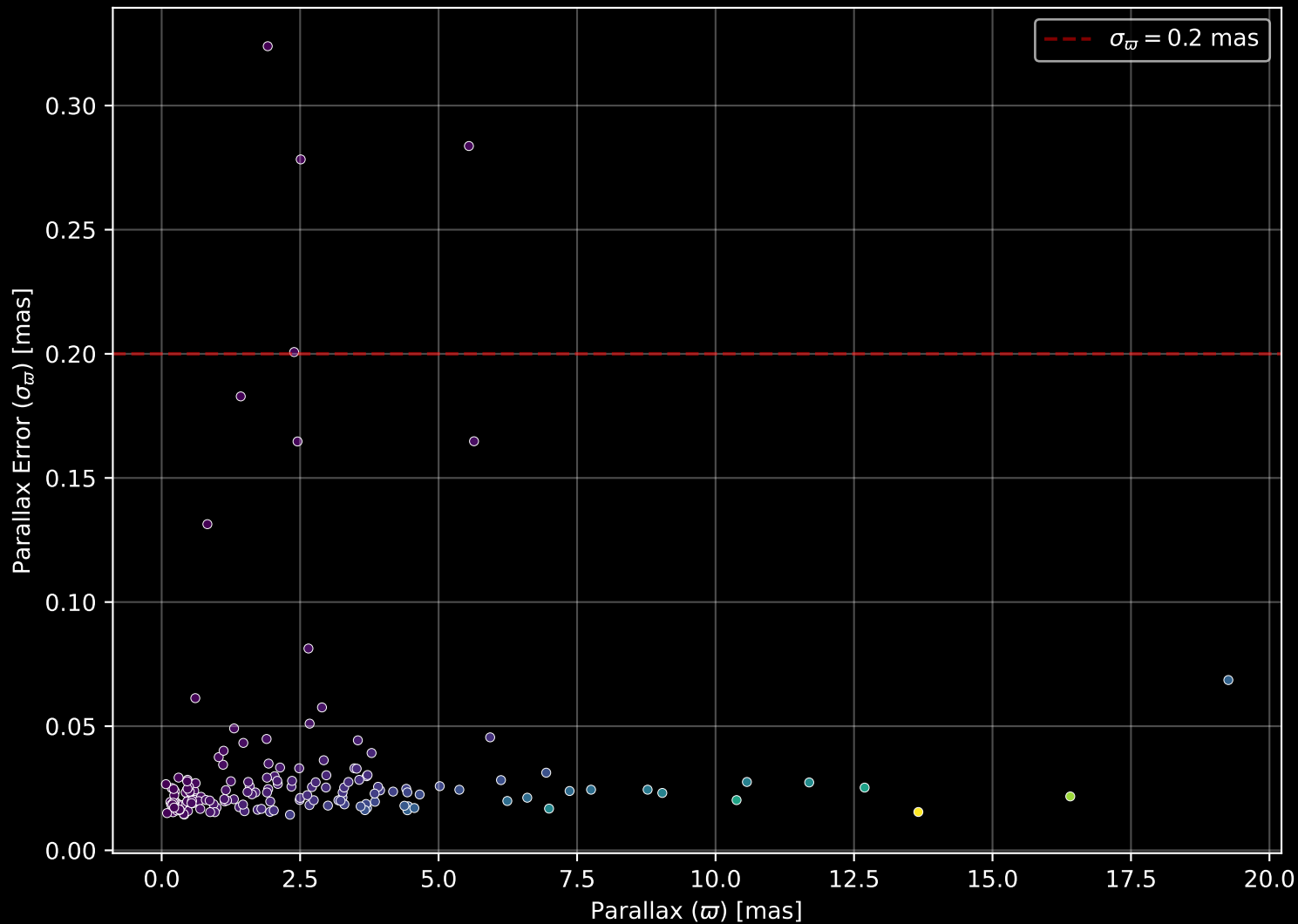
APOGEE DR17 Field: [135-45] Parallax Quality (n= 166)
