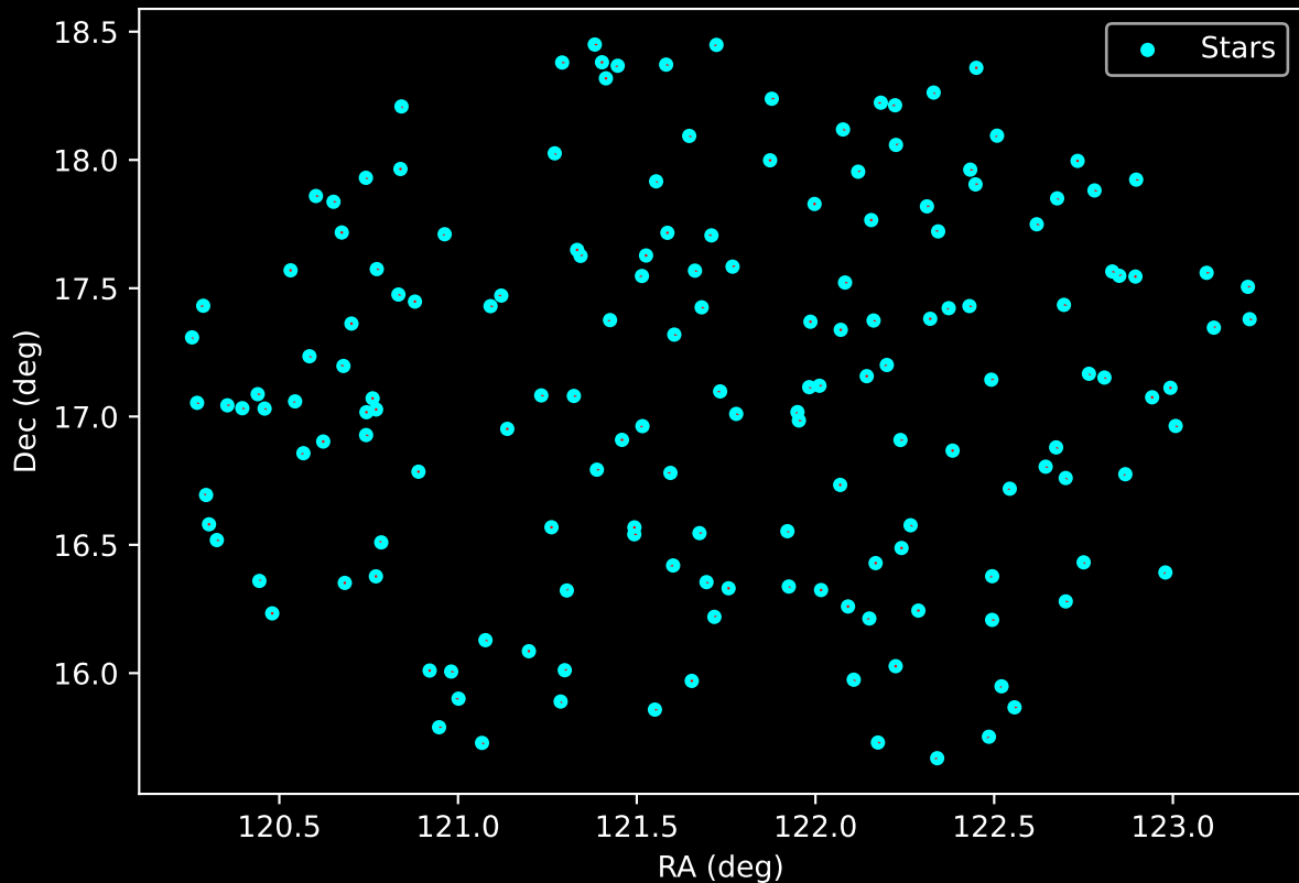
APOGEE DR17 Field: [135-45] Proper Motion Vectors for Gaia Star Field (n= 166)
