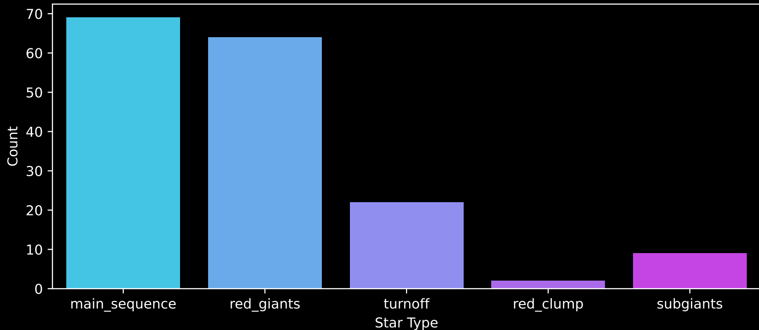
APOGEE DR17 Field: [135-45] Count plot of Star Type
